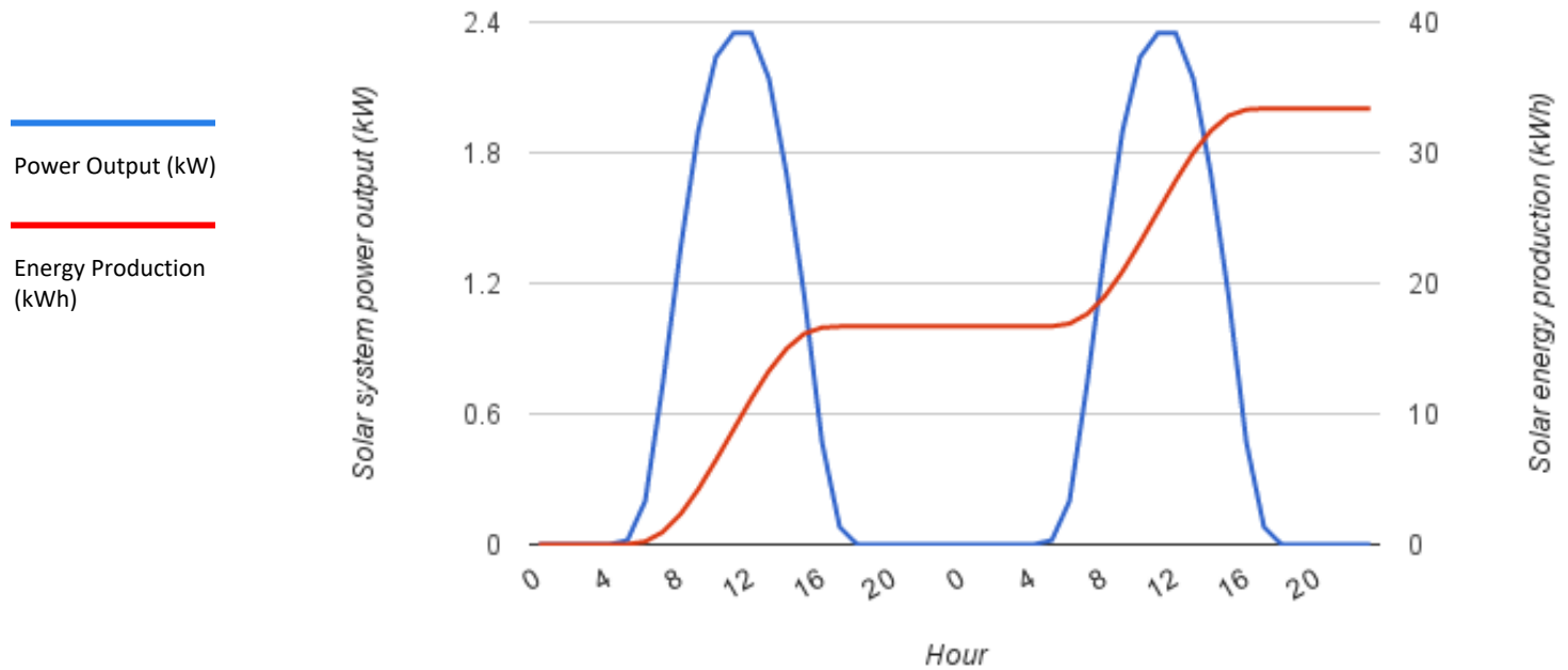
Power output vs energy production for example 2.5kW solar system
